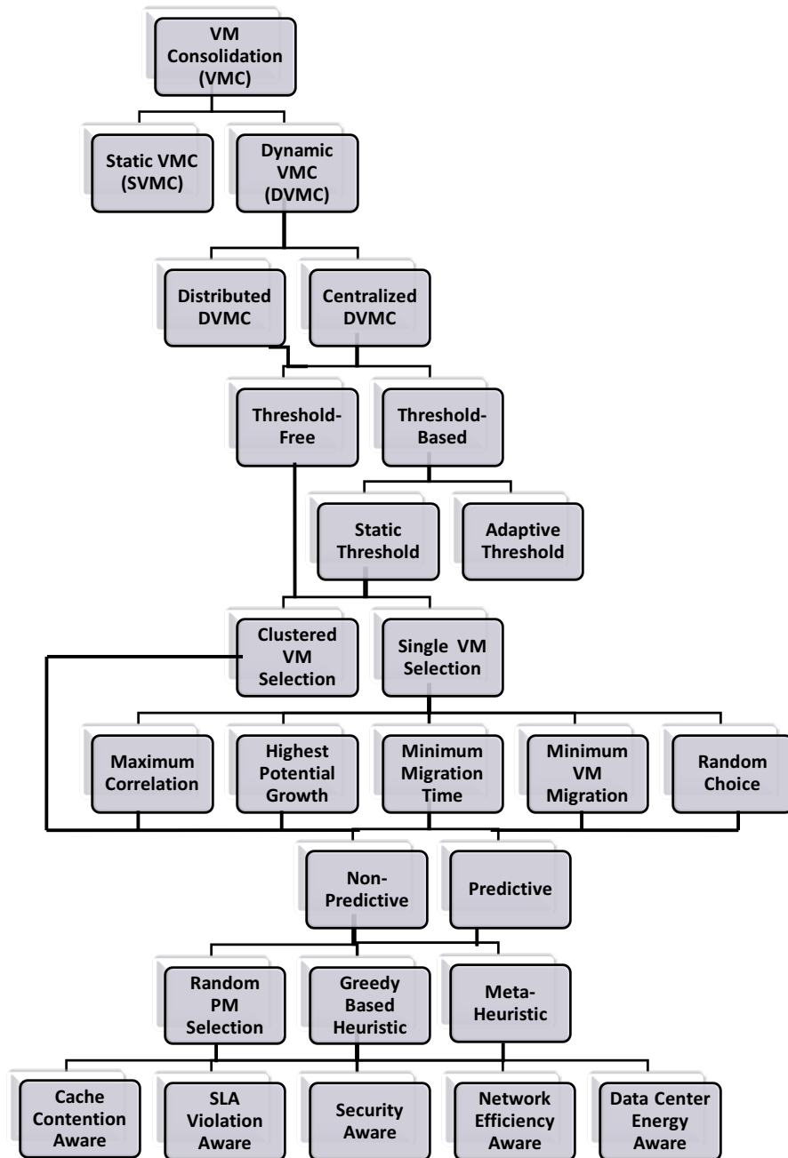
Fig. 3 Classification of DVMC Algorithms
