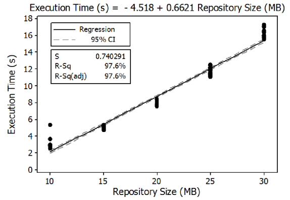
Fig. 6: Execution time of translation for different repository sizes.
